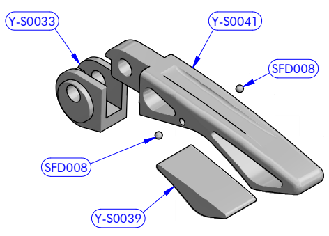
Lever mod. Y-SA002
